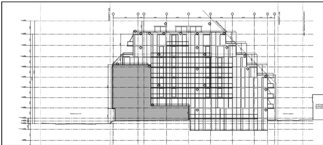
North Elevation
